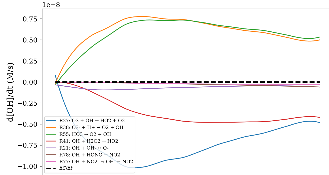
(b) OH [final=0.45 pM]
