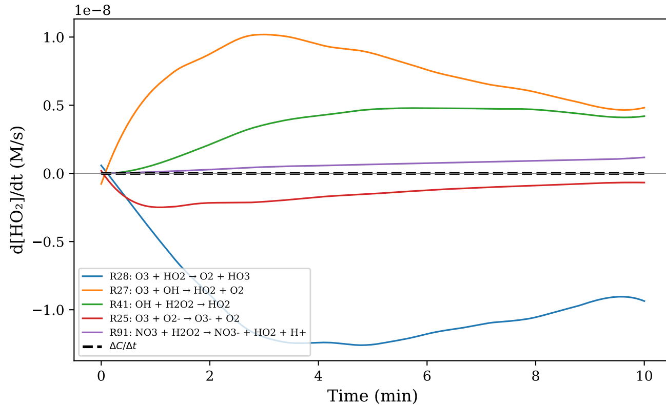
(c) HO 2 [final=317.41 pM]
